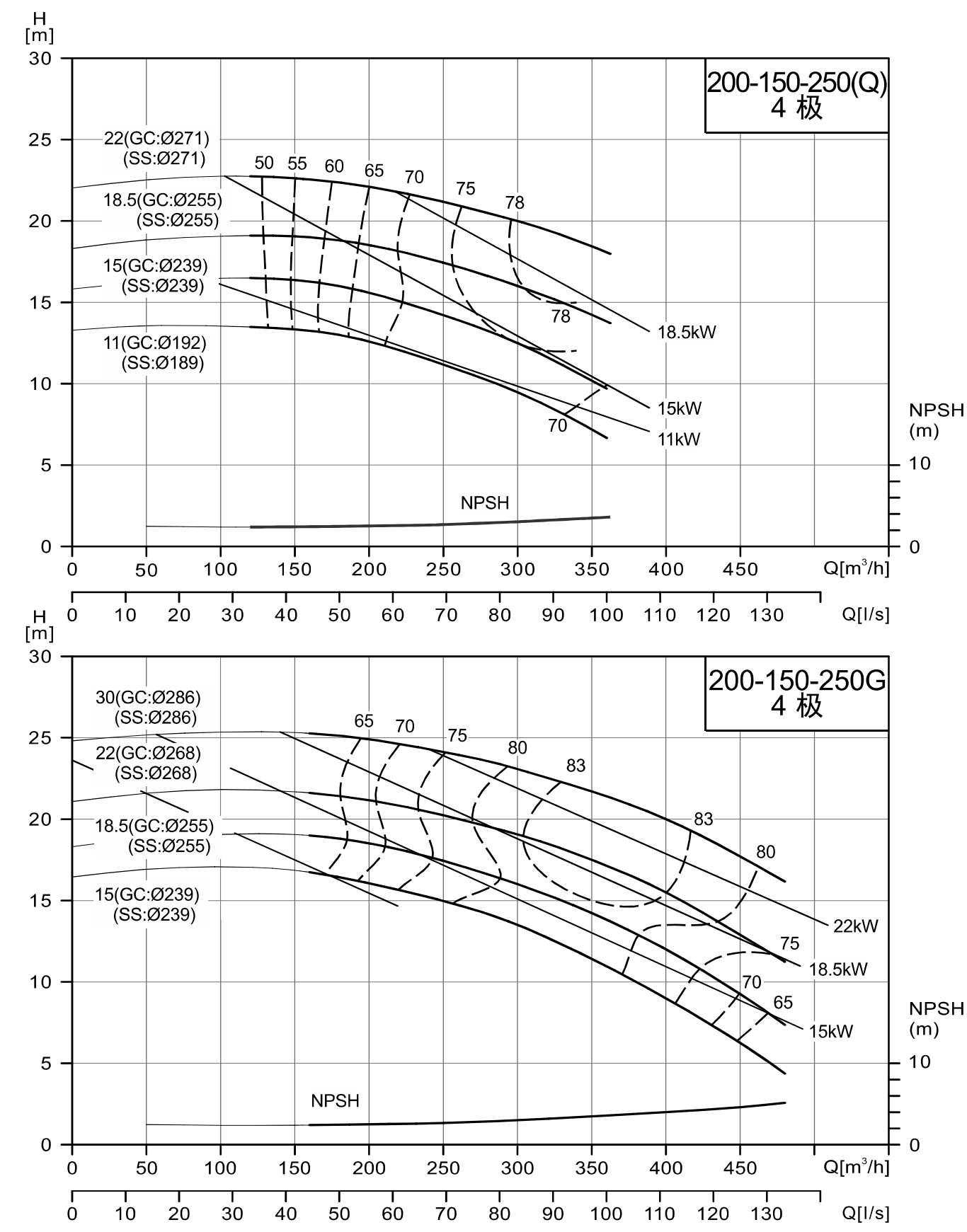
NISO/NIS/NISF200-150-250(Q)/200-150-250G
