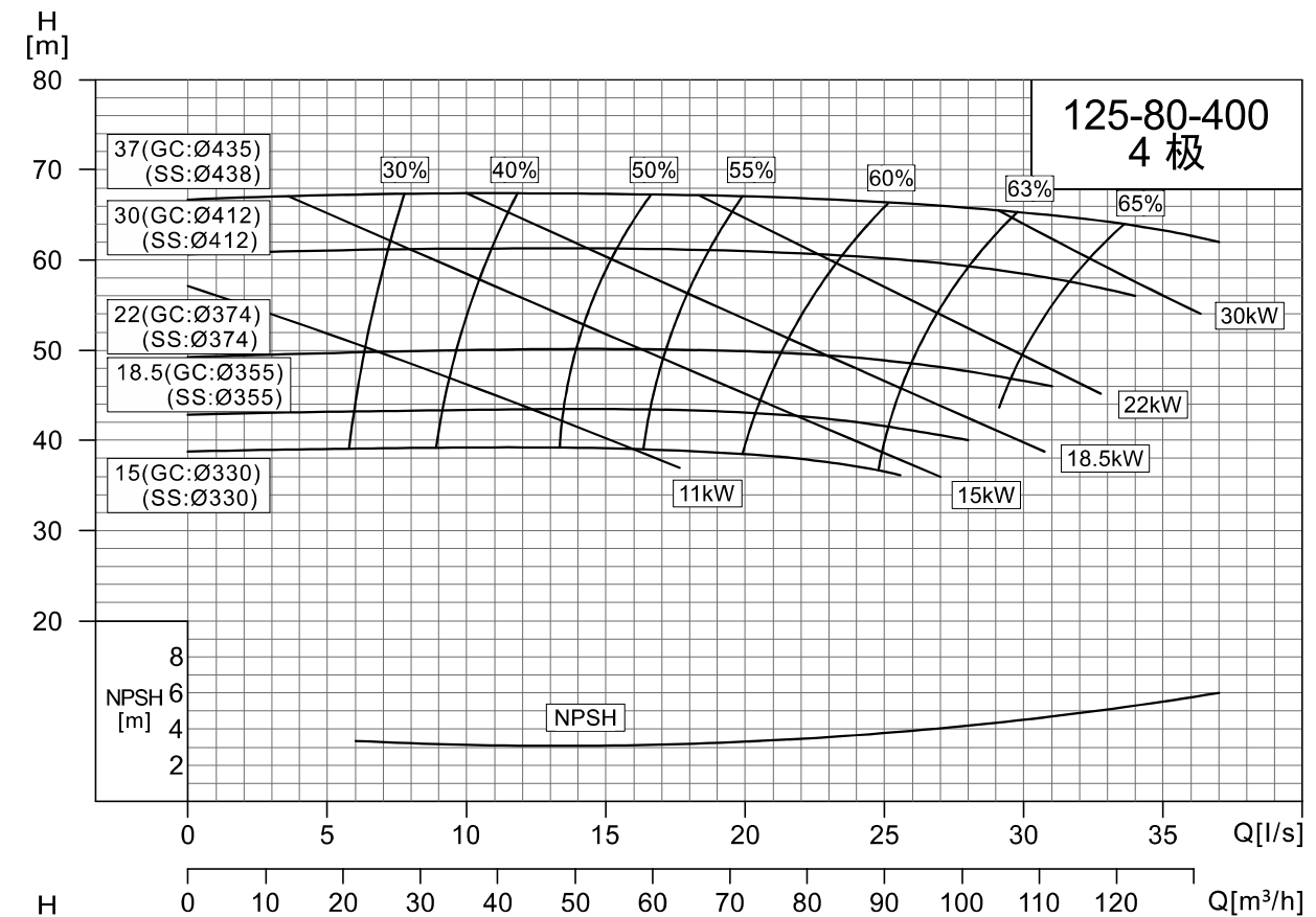
NISO,NIS,NISF125-80-400/125-100-400
