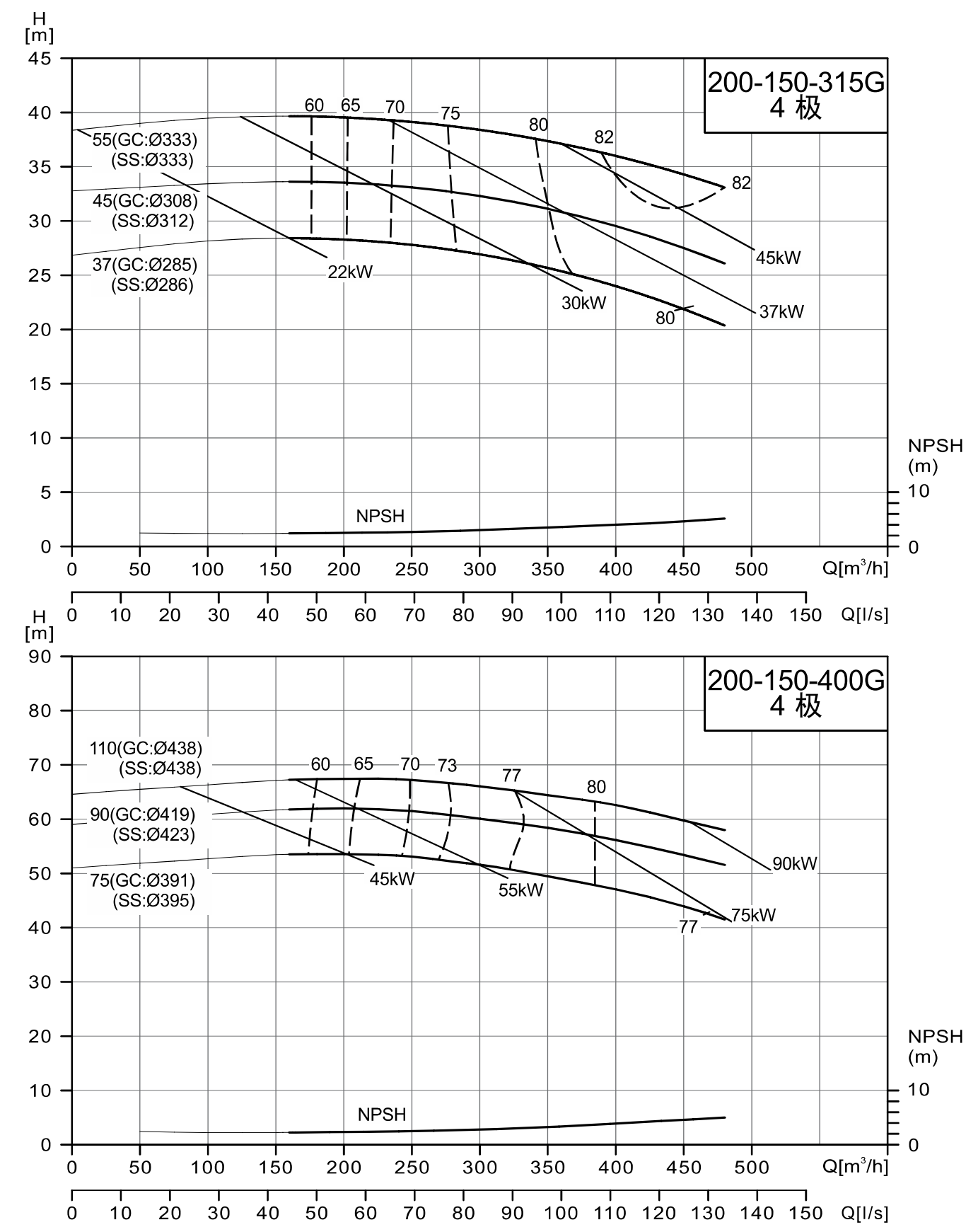
NISO/NIS/NISF200-150-315G/200-150-400G
