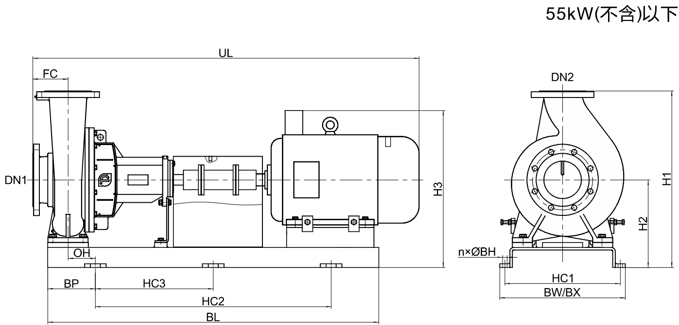
NISO泵组外形尺寸图(膜片联轴器结构)
