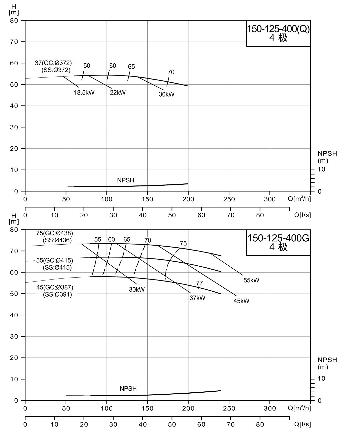
NISO/NIS/NISF150-125-400(Q)/150-125-400G
