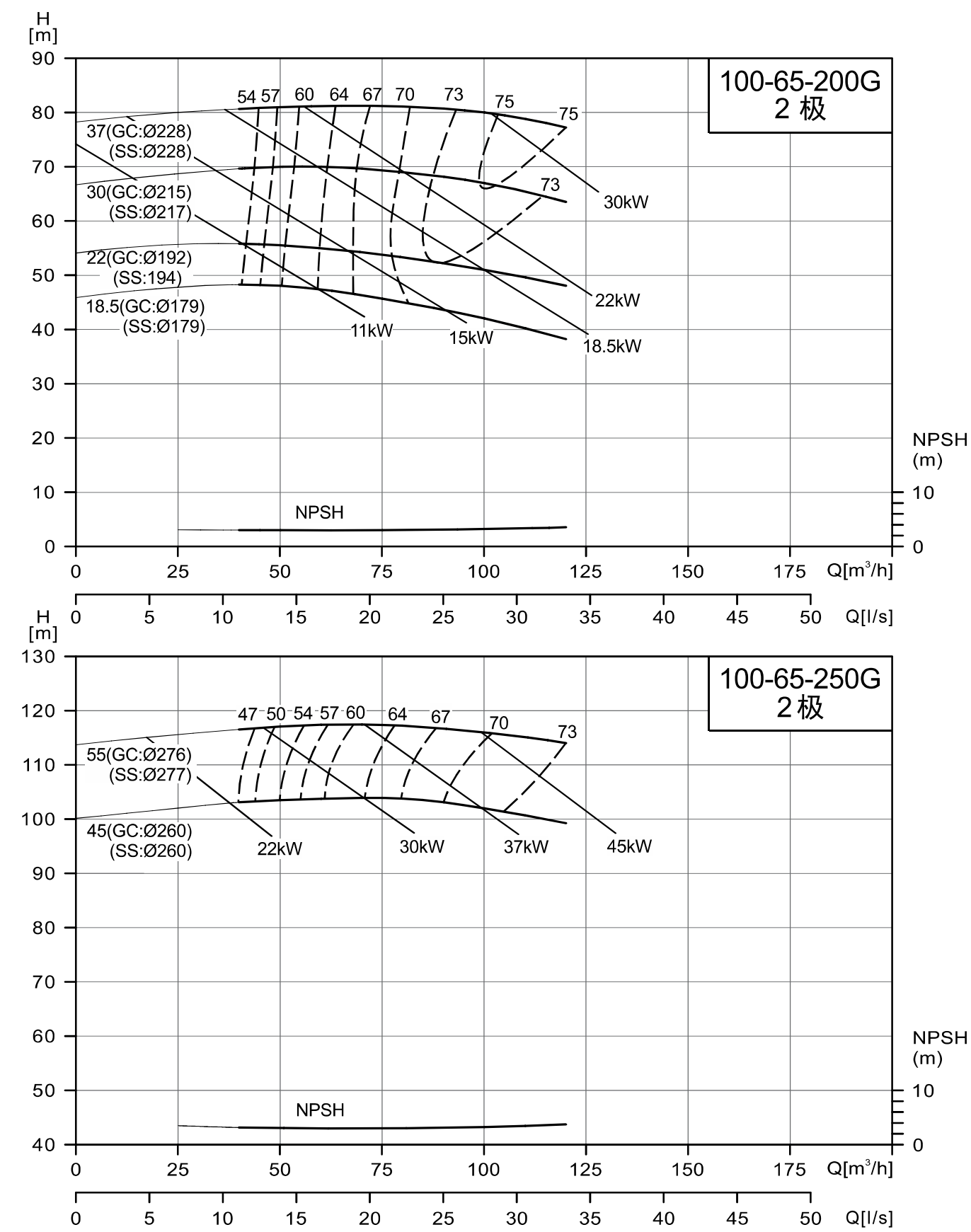
NISO/NIS/NISF100-65-200G/100-65-250G
