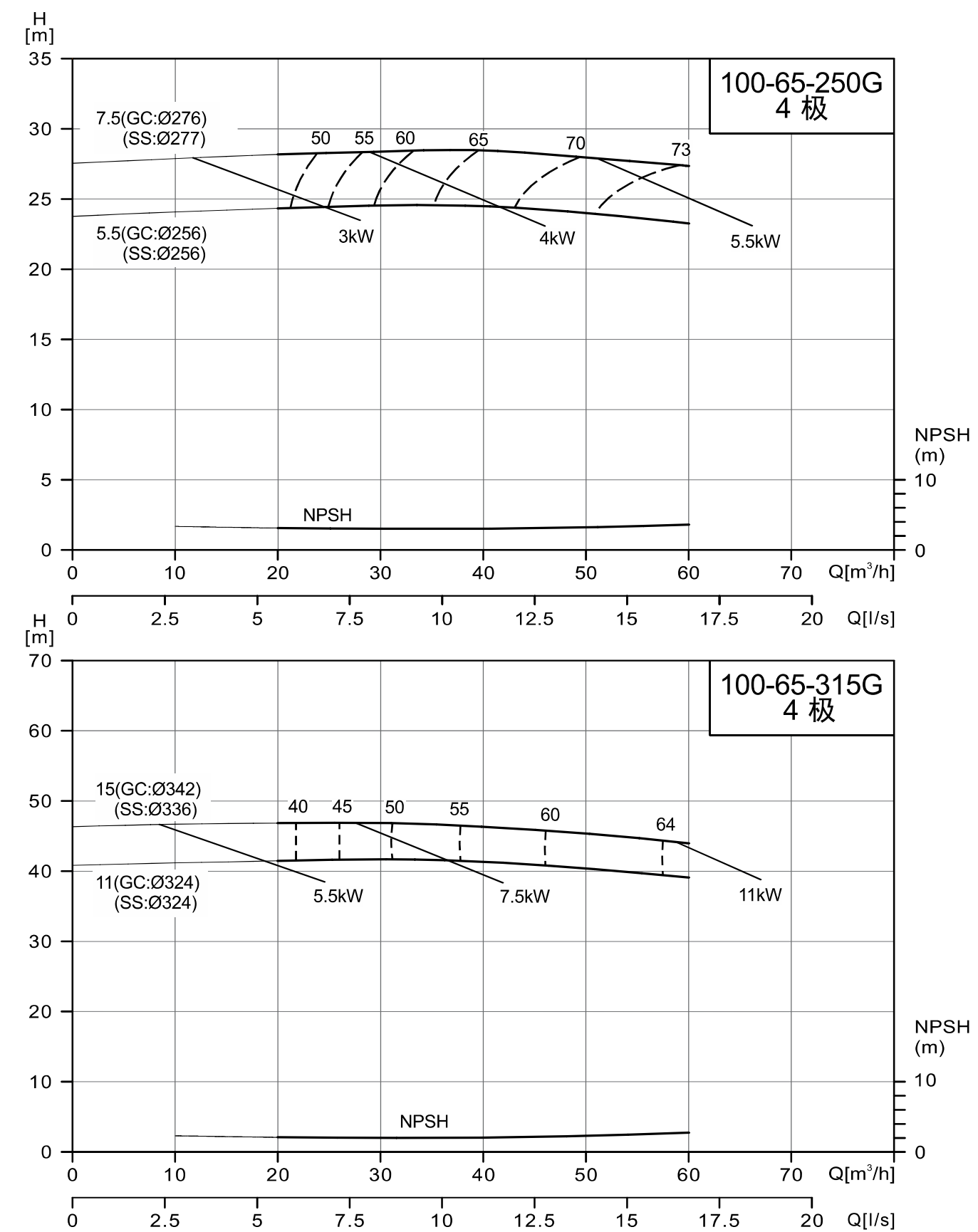
NISO/NIS/NISF100-65-250G/100-65-315G
