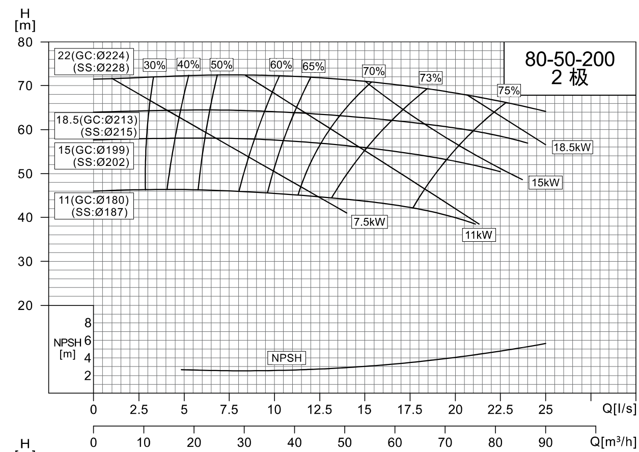
NISO,NIS,NISF80-50-200/80-50-250
