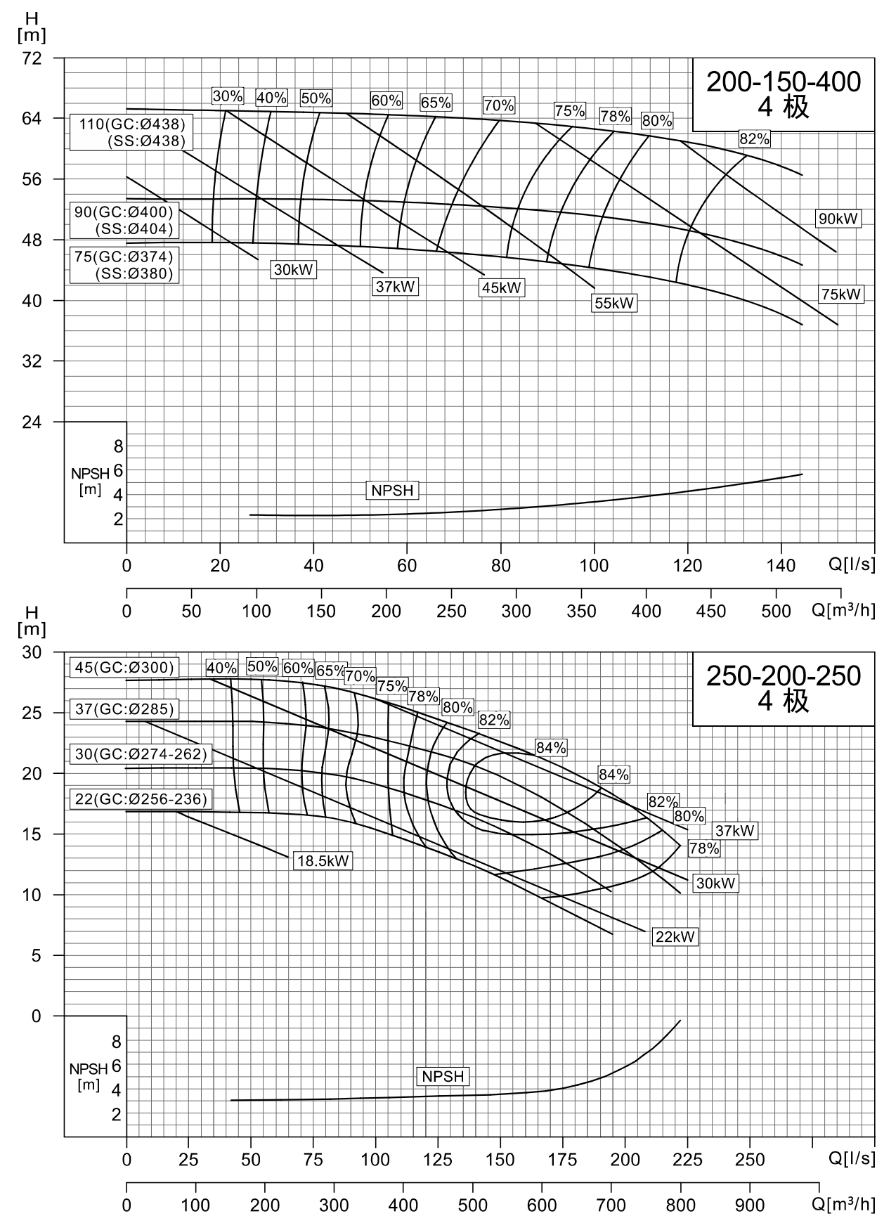
NISO,NIS,NISF200-150-400/250-200-250
