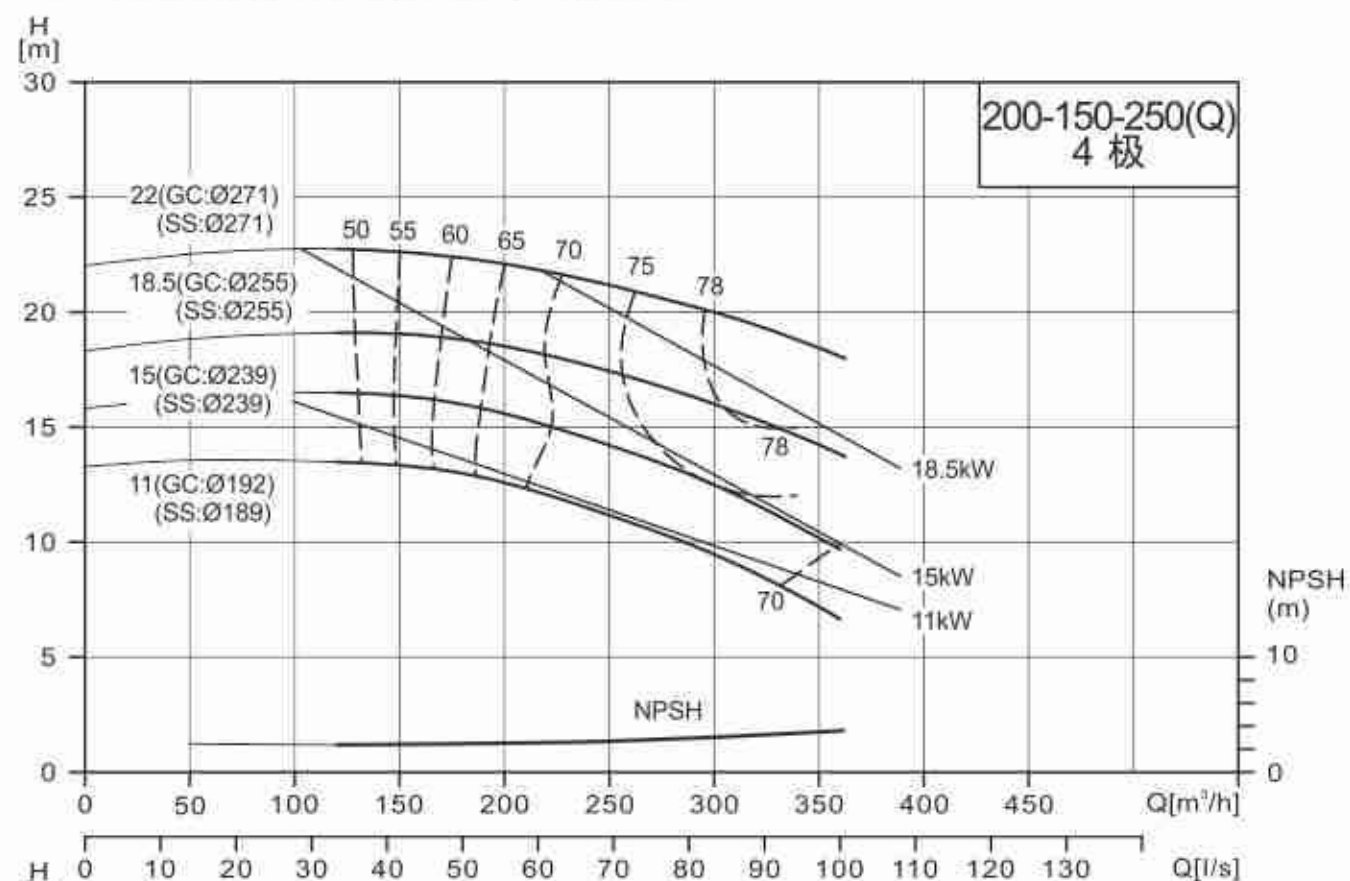
NISO/NIS/NISF200-150-250(Q)/200-150-250G
