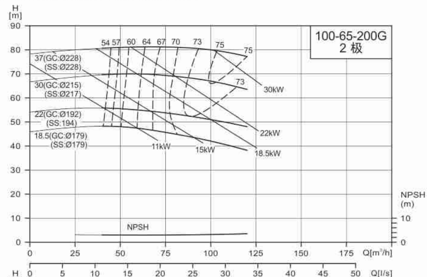
NISO/NIS/NISF100-65-200G/100-65-250G
