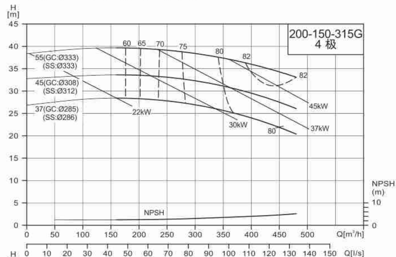
NISO/NIS/NISF200-150-315G/200-150-400G
