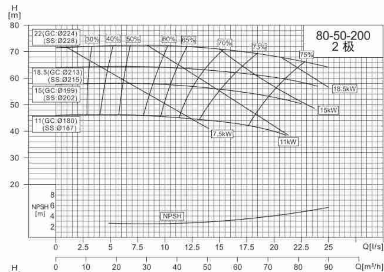
NISO,NIS,NISF80-50-200/80-50-250
