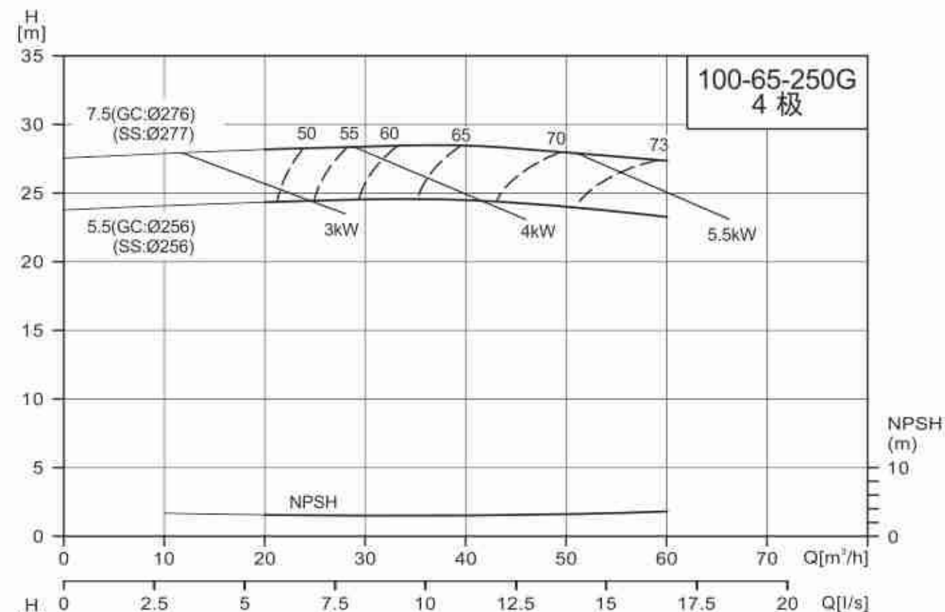
NISO/NIS/NISF100-65-250G/100-65-315G
