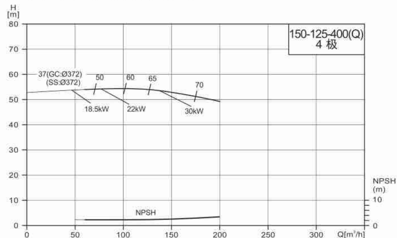
NISO/NIS/NISF150-125-400(Q)/150-125-400G
