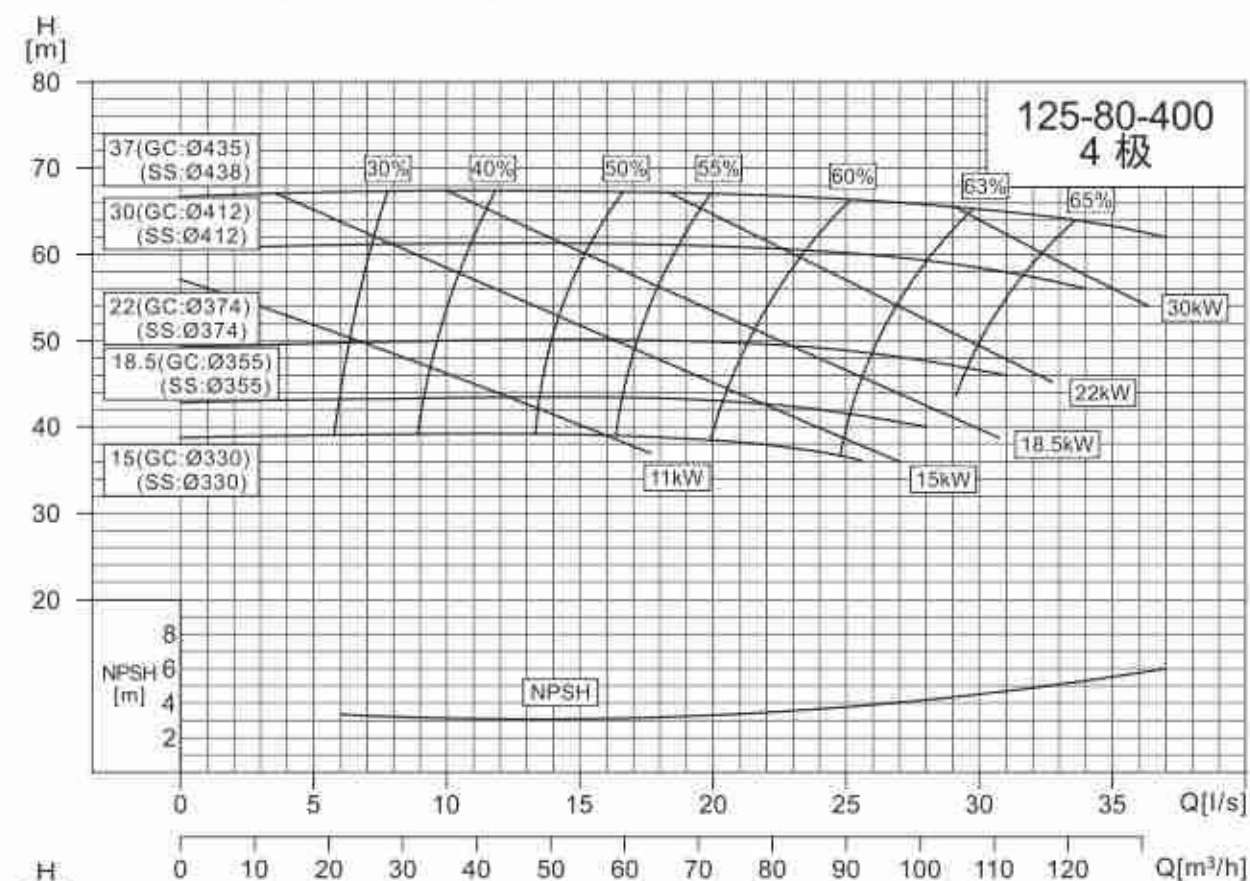
NISO,NIS,NISF125-80-400/125-100-400
