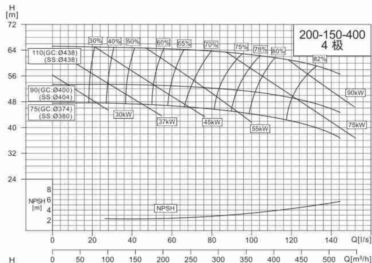
NISO,NIS,NISF200-150-400/250-200-250
